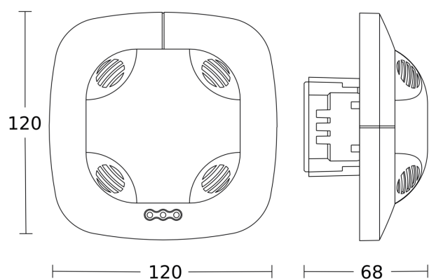
Dimension Drawing 1
